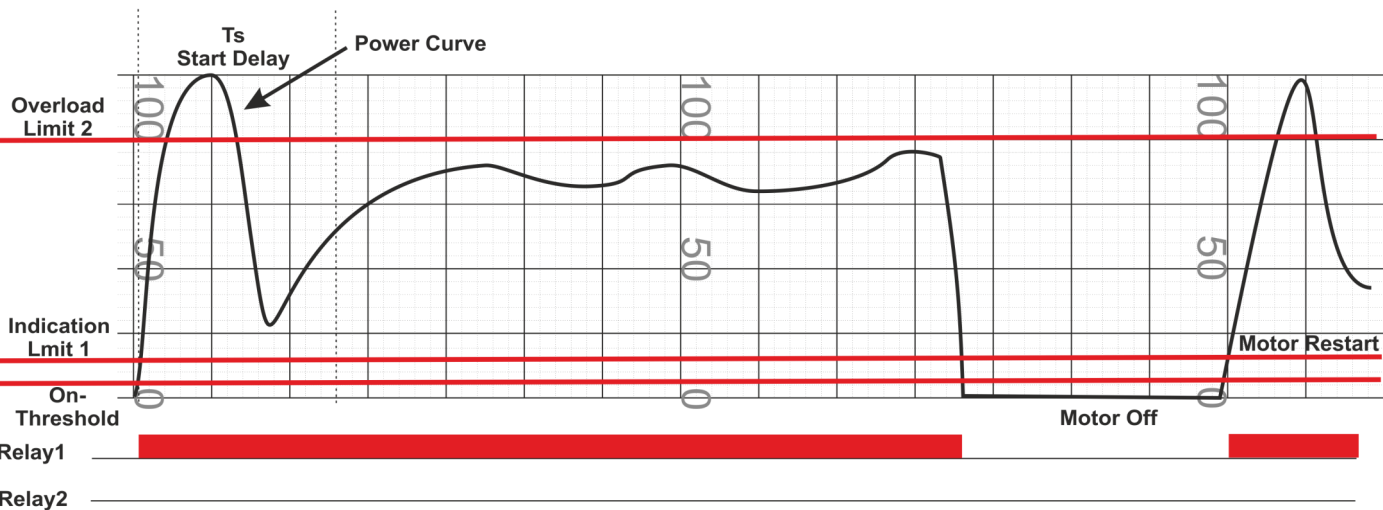
Example #3 Dual Max. Load Power (Torque) Curve.
