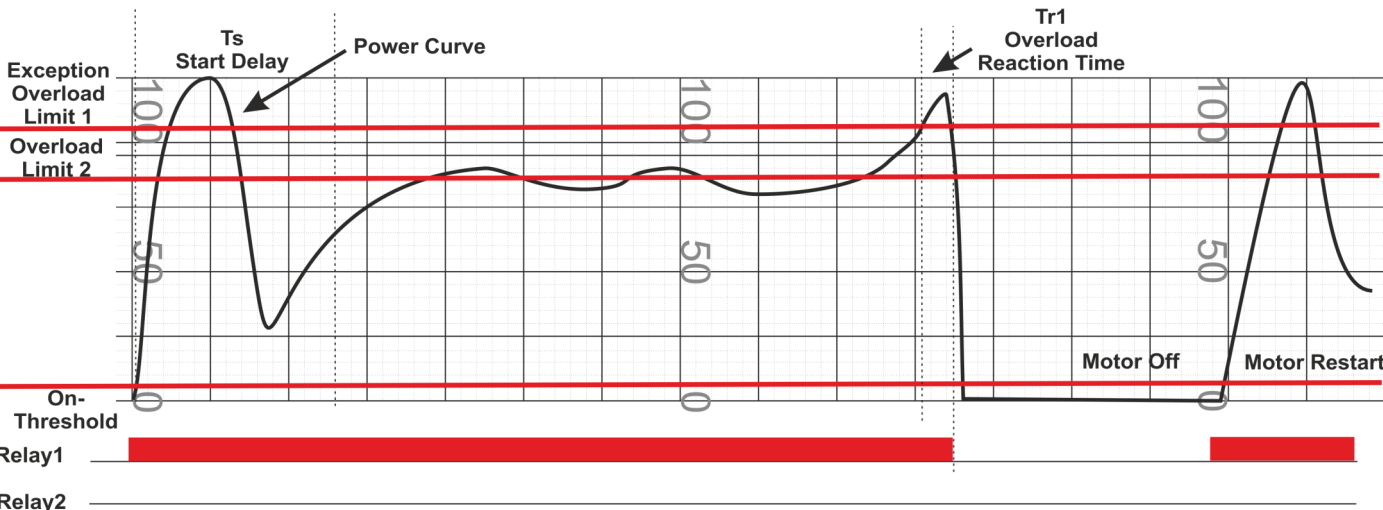
Example #2 Dual Max. Load Power (Torque) Curve.
